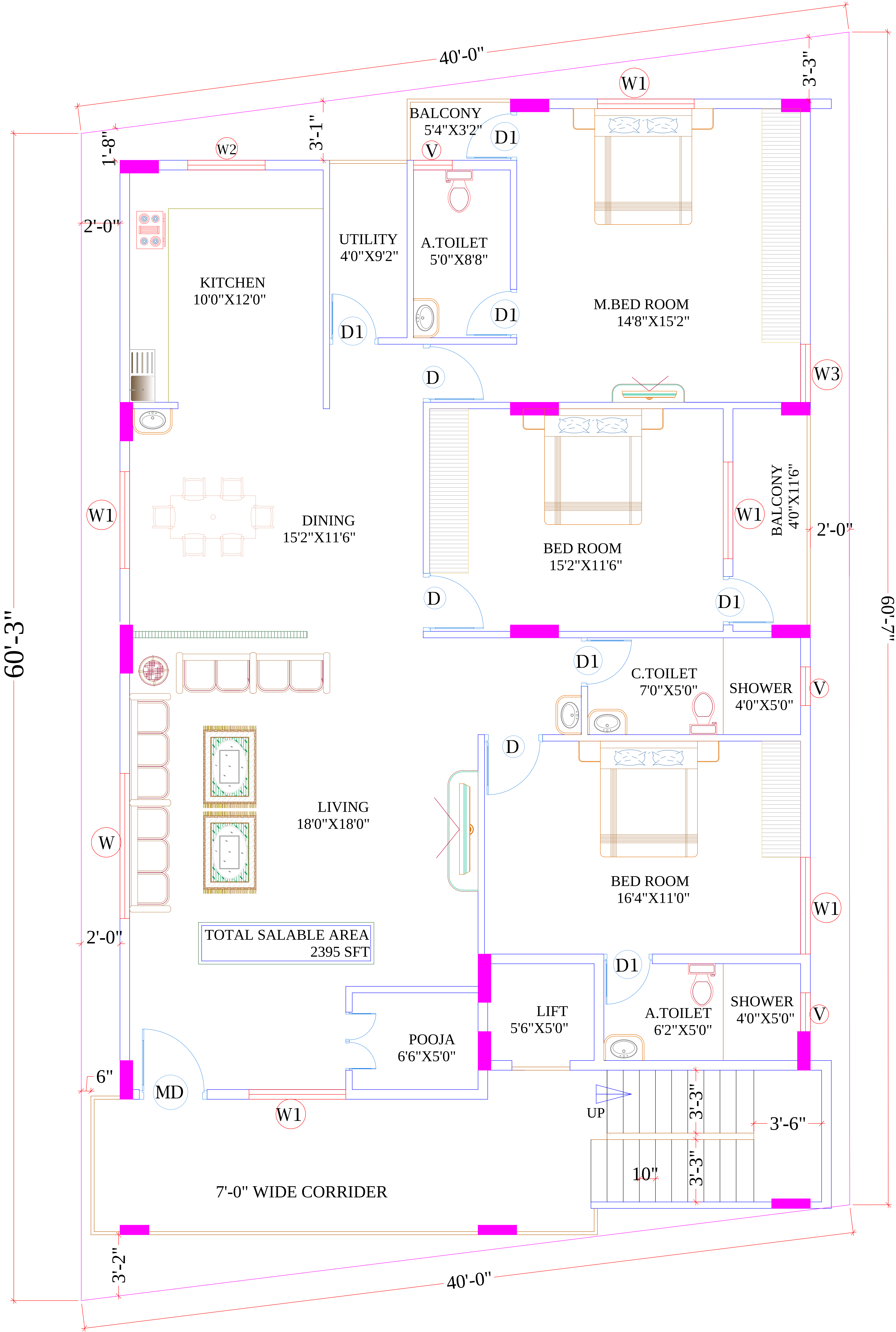
N O R T H B Y R O A D TYPICAL FLOOR PLAN
